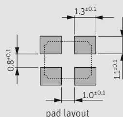
pad layout
