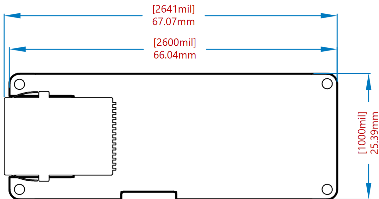
Board dimensions
