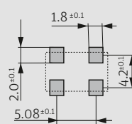
pad layout
