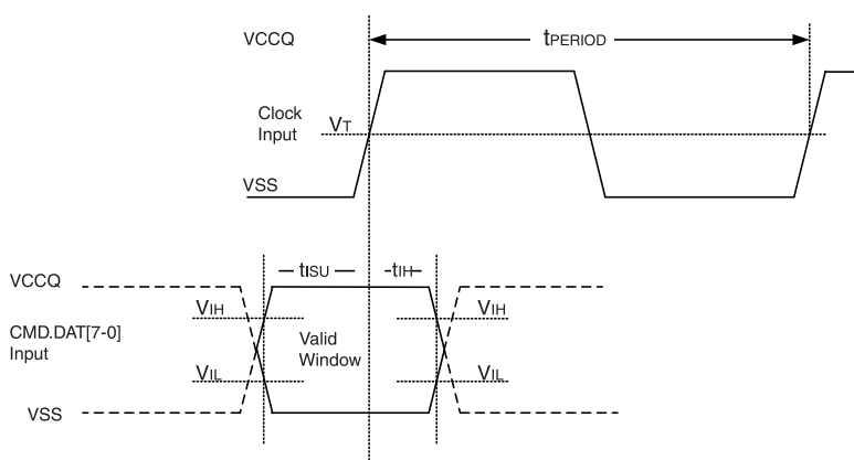
Figure 7.4 HS200 Device Input Timing
