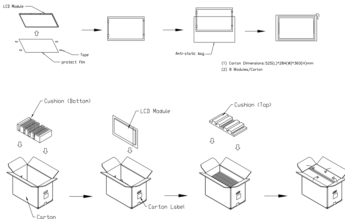
Figure. 7-1 Packing
