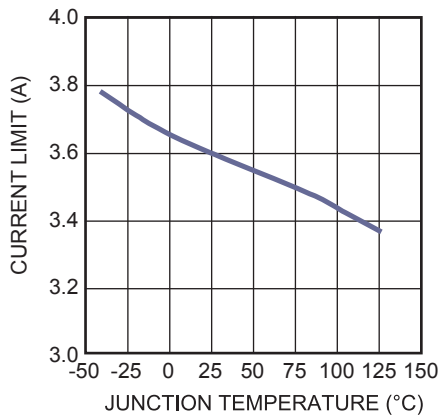
Boost Current Limit vs. Junction Temperature
