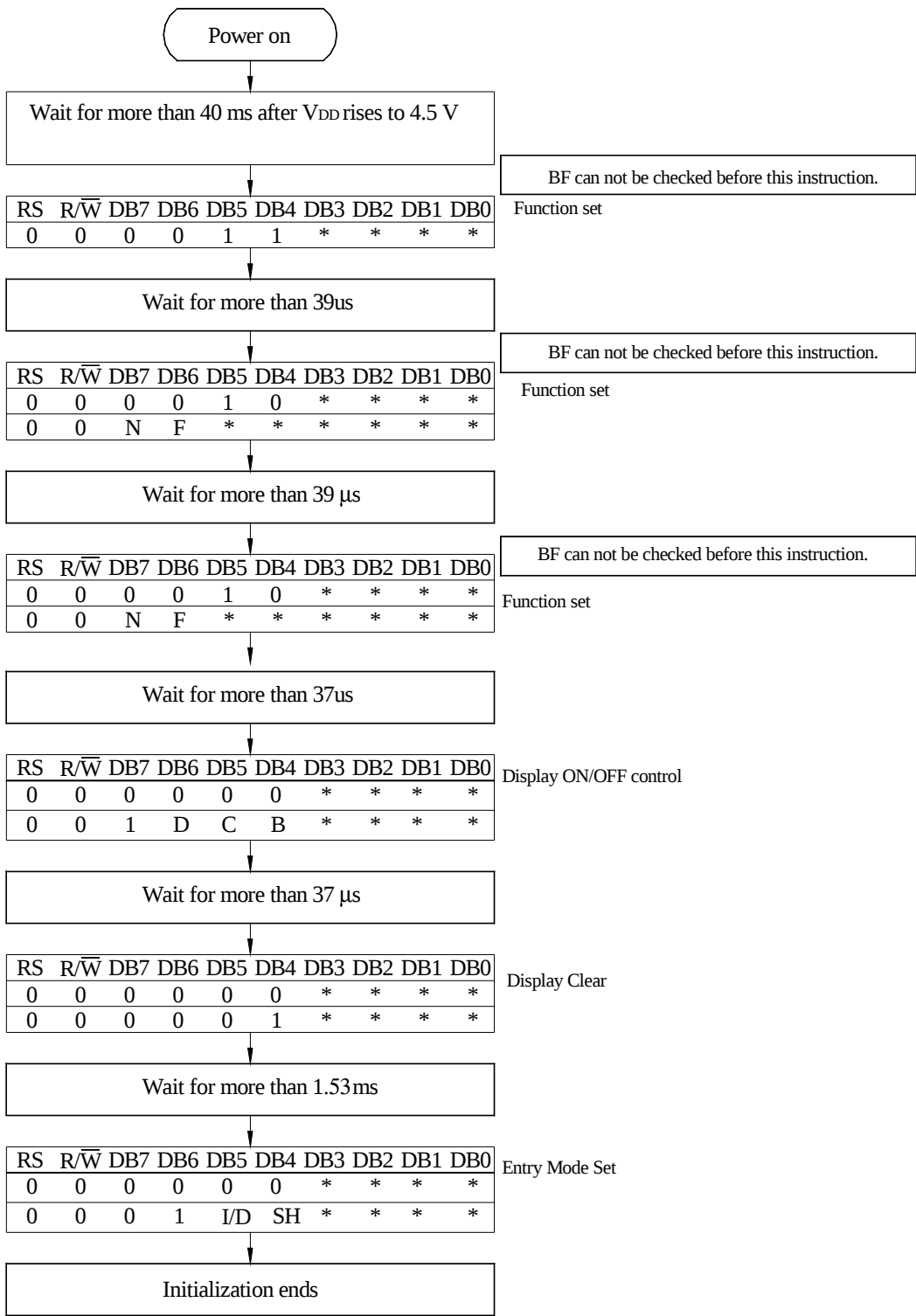
4-Bit Ineterface
