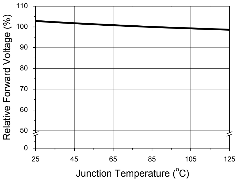
Fig 6. Junction Temperature vs. Forward Voltage, I_F=0.72A
