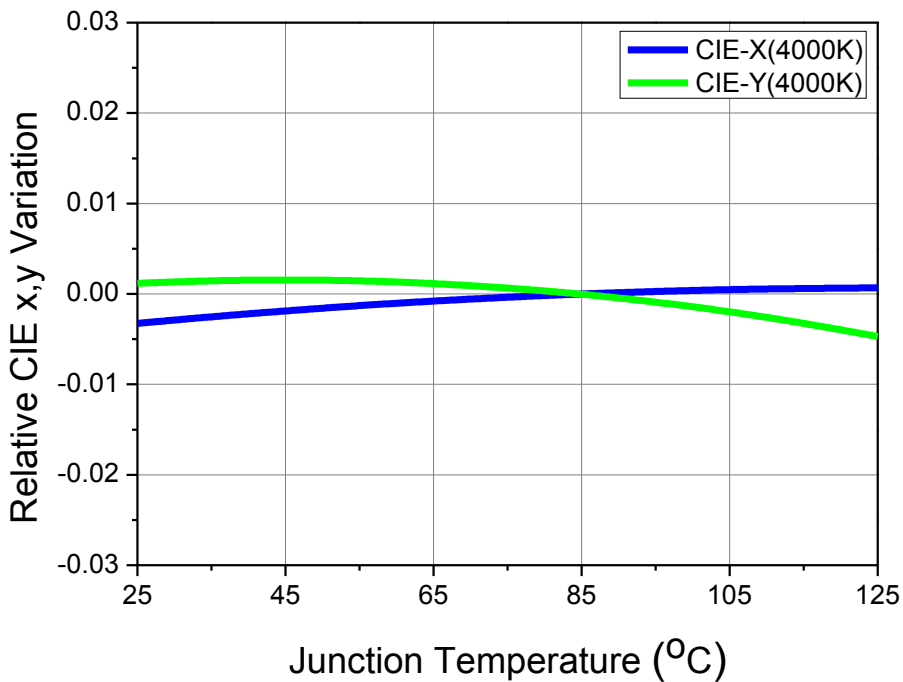
Fig 8. Junction Temperature vs. CIE x,y Shift, I_F=0.72A (4000K)
