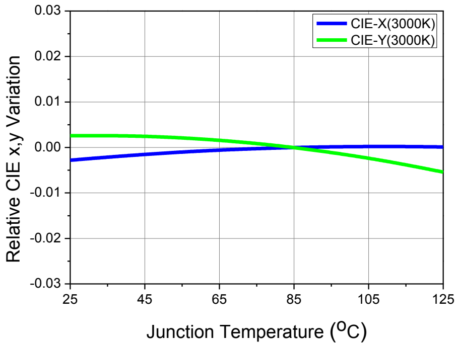
Fig 9. Junction Temperature vs. CIE x,y Shift, I_F=0.72A (3000K)
