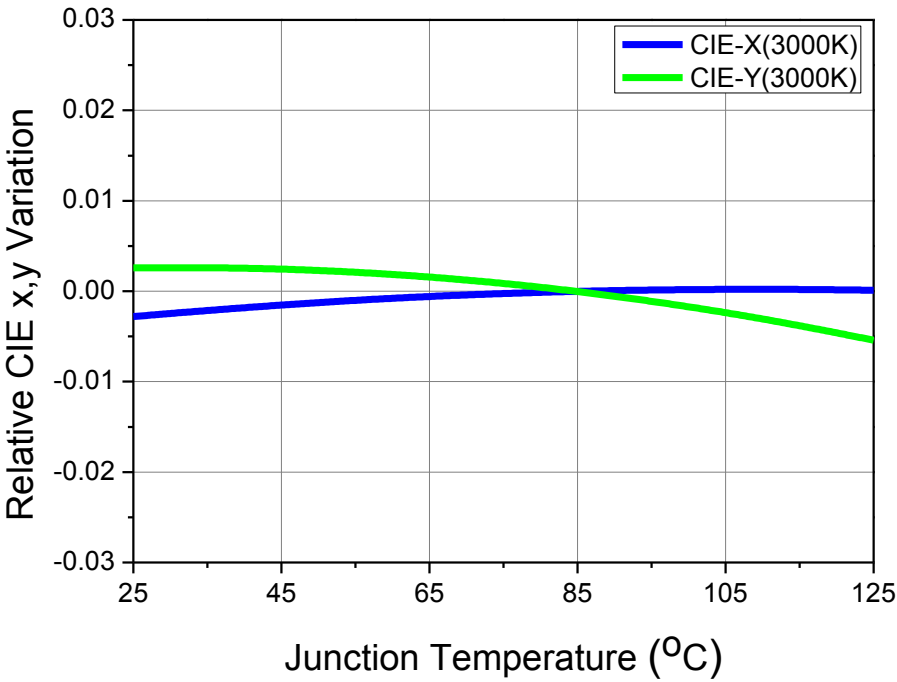
Fig 9. Junction Temperature vs. CIE x,y Shift, I_F=0.29A (3000K)
