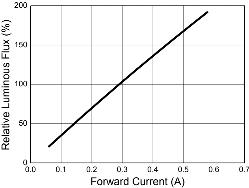
Fig 4. Forward Current vs. Relative Luminous Flux, T_j=85^{\circ}\text{C}
