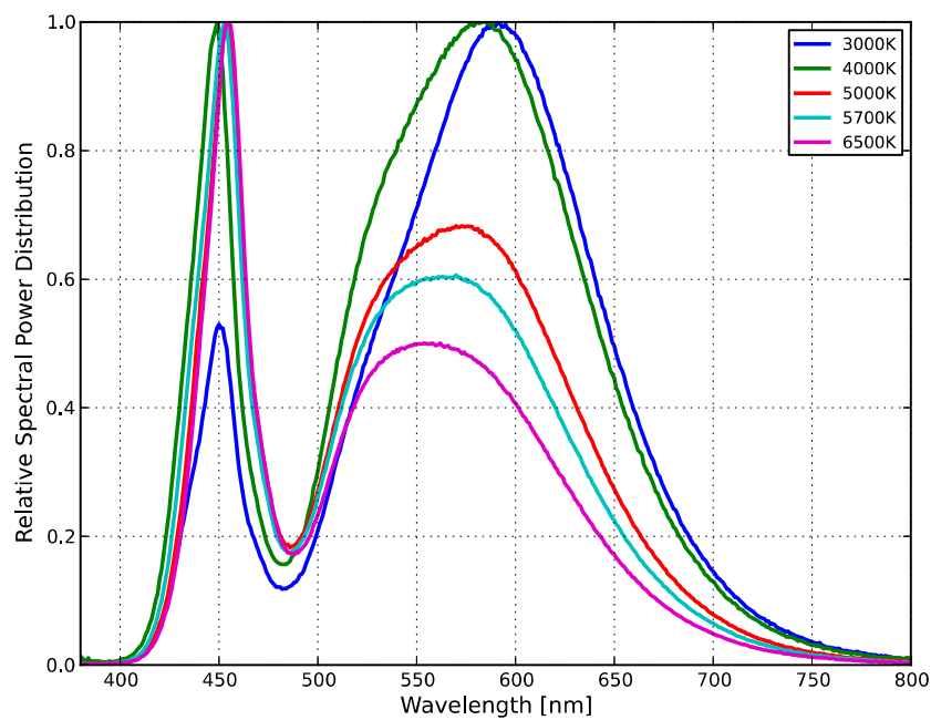
Figure 1a. Typical normalized power vs. wavelength for L1T2-xx700000000000 at 700mA, T_j = 85^\circ\text{C} .
