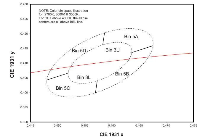
Figure 7. Color space definition for LUXEON TX.
