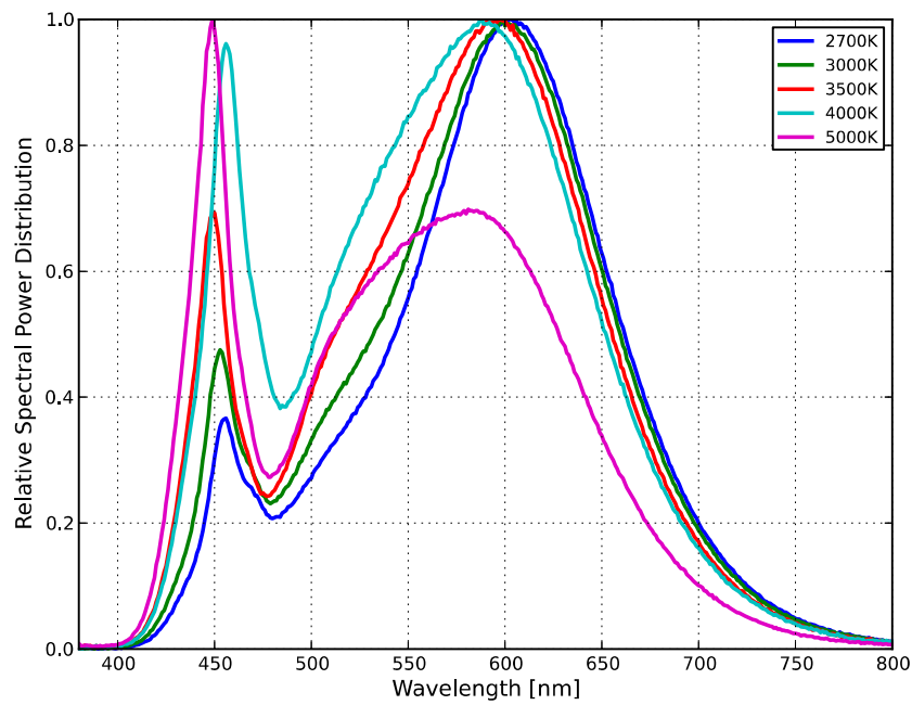
Figure 1b. Typical normalized power vs. wavelength for L1T2-xx800000000000 at 700mA, T_j = 85^\circ\text{C} .
