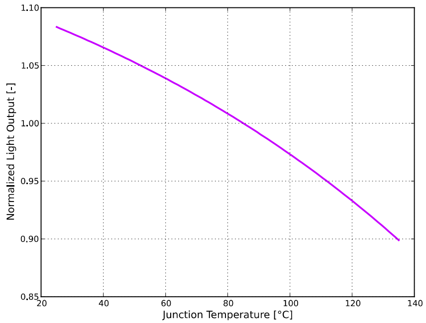
Figure 2g. Typical normalized light output vs. junction temperature for LUXEON CZ Violet at 350mA.
