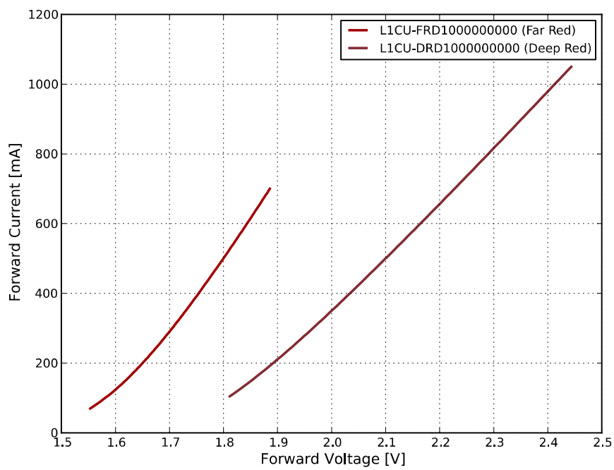
Figure 4a. Typical forward current vs. forward voltage for LUXEON CZ Far Red and Deep Red at T_j=85^{\circ}\text{C} .
