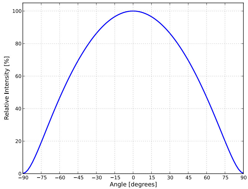
Figure 5. Typical radiation pattern for L150-xxxx50xx000x0 at test current, T j =25°C.
