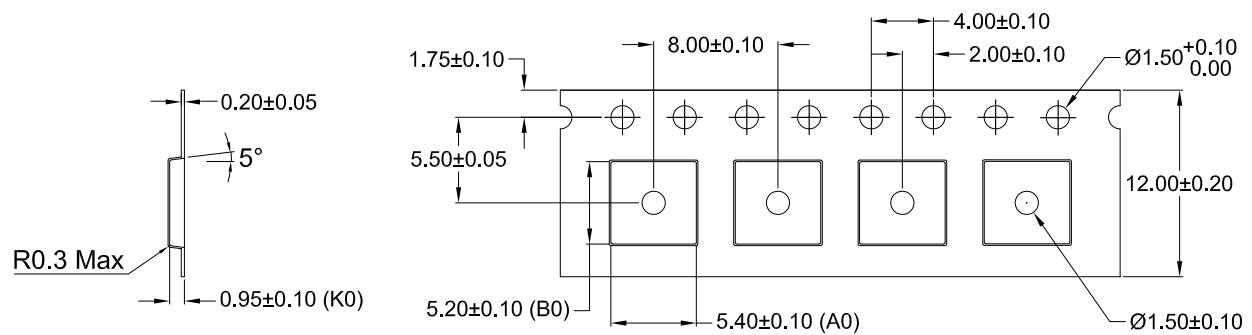
Figure 11. Pocket Tape dimensions for LUXEON SunPlus 5050.
