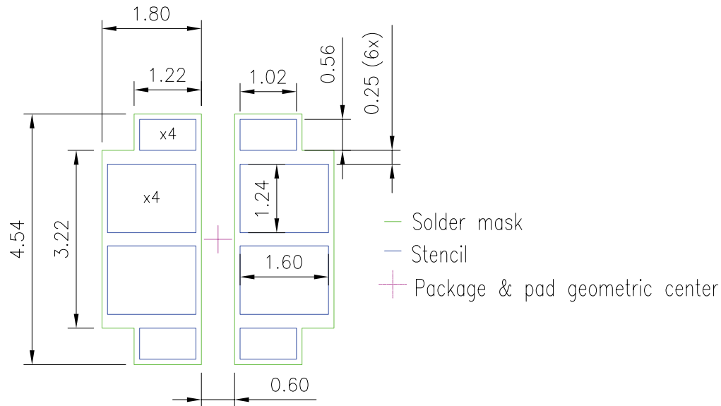
Figure 10. Recommended PCB solder pad layout for LUXEON SunPlus 5050.
