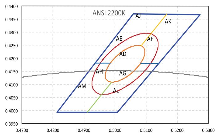
Figure 8a. Color bin structure for LUXEON 3014 2200K, hot-color targeted at T j =65°C.
