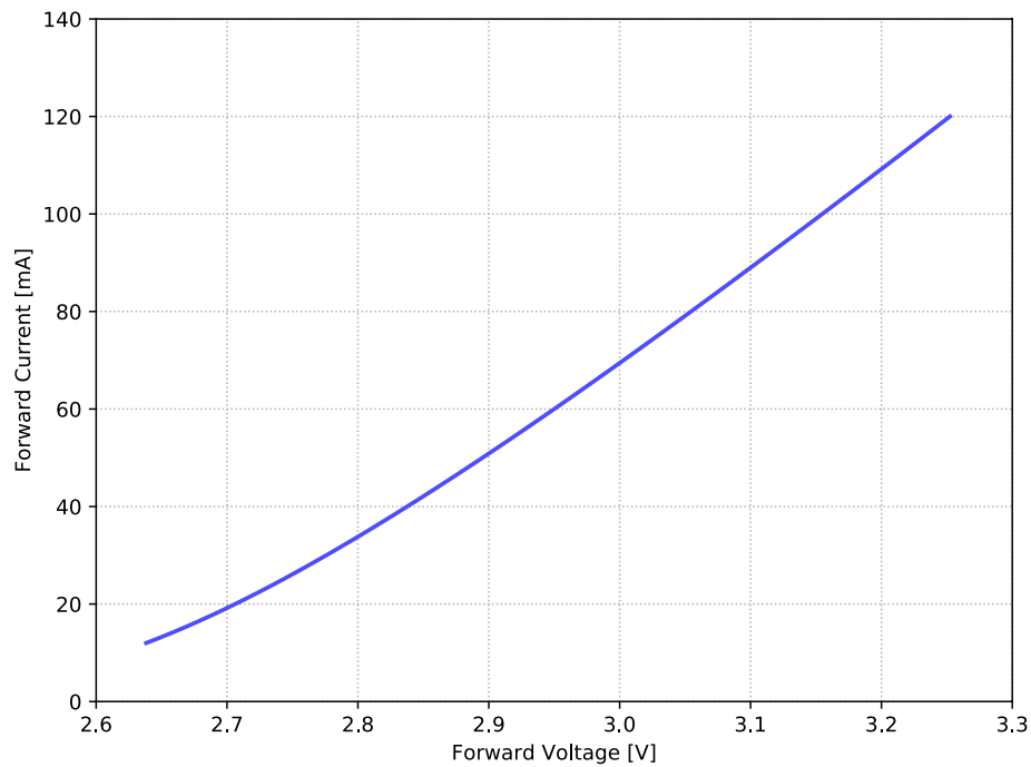
Figure 4. Typical forward current vs. forward voltage for L130-xxxxxx1400001 at T j =25°C.
