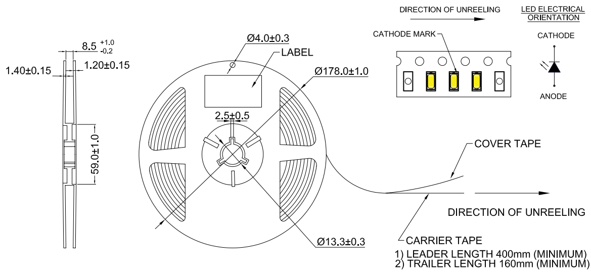
Figure 13. Reel dimensions for LUXEON 3014.
