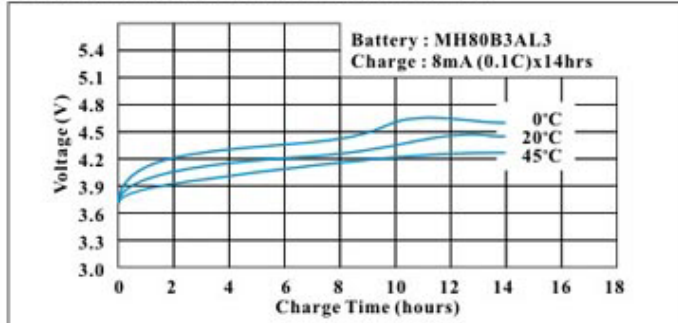
Typical Quick Charge Characteristics (Button Cell)
