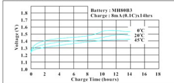
Typical Quick Charge Characteristics (Button Cell)
