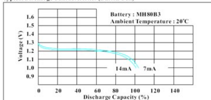
Typical Discharge Characteristics (Button Cell)
