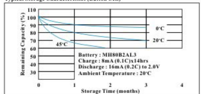
Typical Storage Characteristics (Button Cell)
