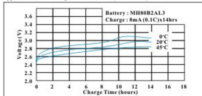
Typical Quick Charge Characteristics (Button Cell)
