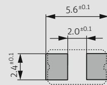
pad layout
