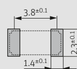
pad layout
