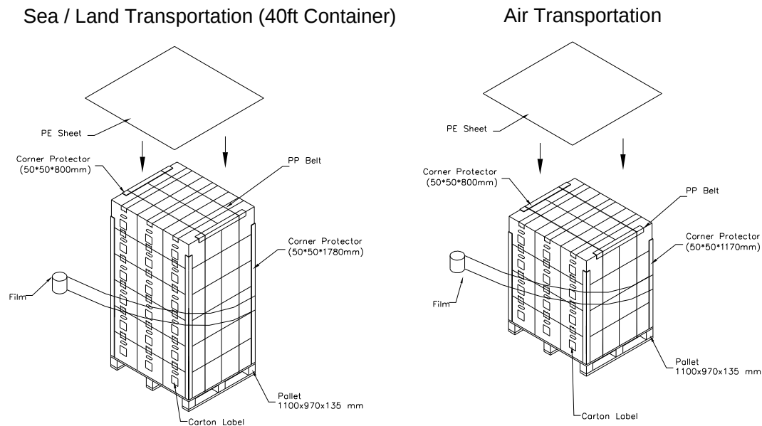
Figure. 7-2 Packing
