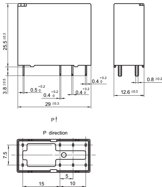
Outline Dimensions
