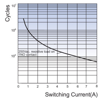
ELECTRICAL ENDURANCE
