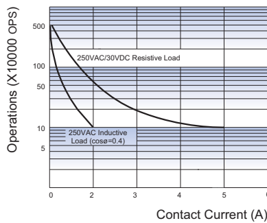
ENDURANCE CURVE
