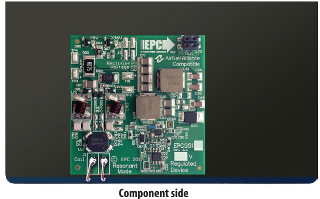
Photo of the EPC9515 receiver board.
