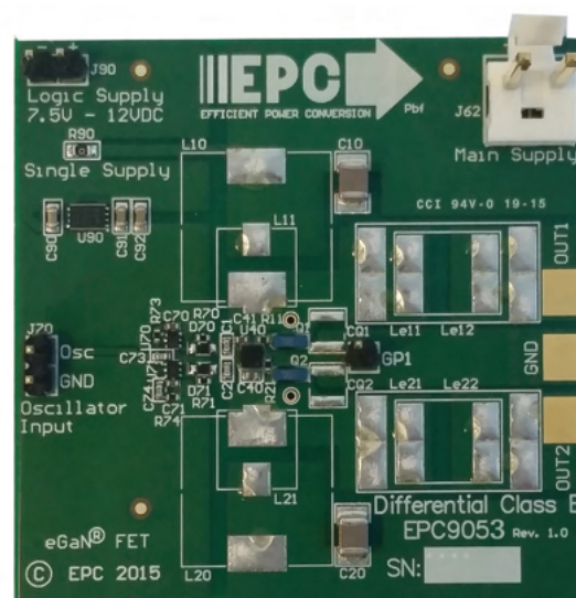
EPC9053 amplifier board photo
