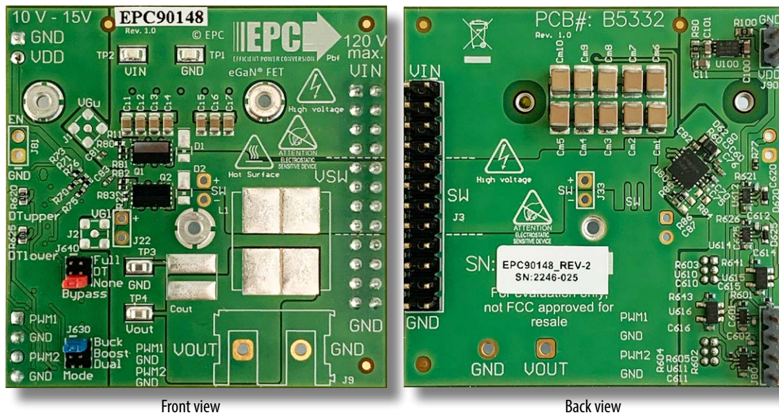
EPC90148 development board
