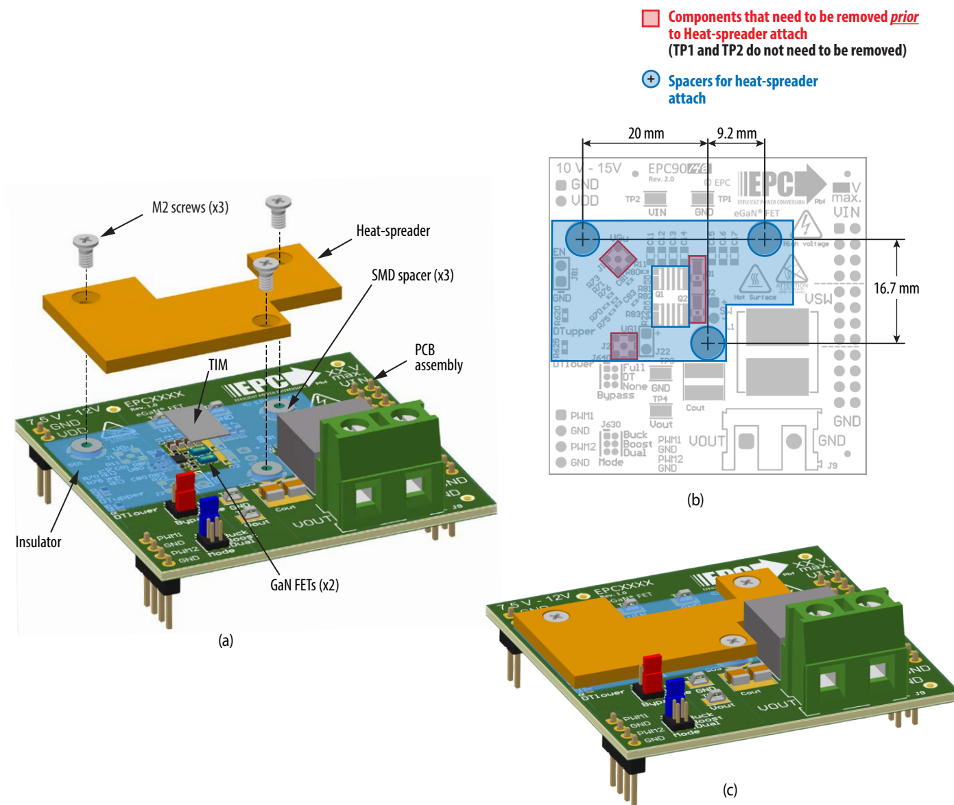
Figure 9: Details for attaching a heatsink to the development board. (a) 3D perspective, (b) top view details, (c) Assembled view with heat-spreader attached.
