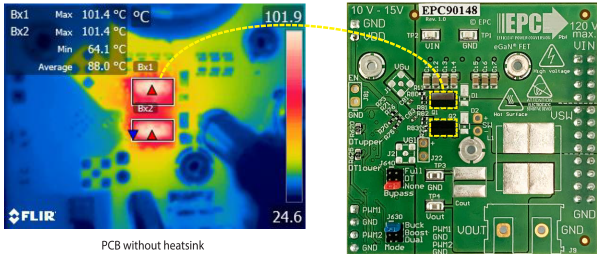
Figure 16: Measured thermal image and thermal couple readings of case temperature when operating under the following conditions: f_s = 100 \text{ kHz} , I_{OUT} = 30 \text{ A} output, 25^\circ\text{C} ambient and high air flow
