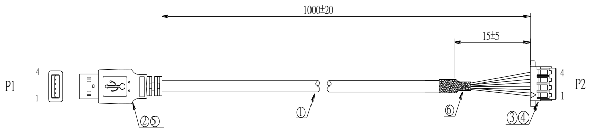
PIN ASSIGNMENT
