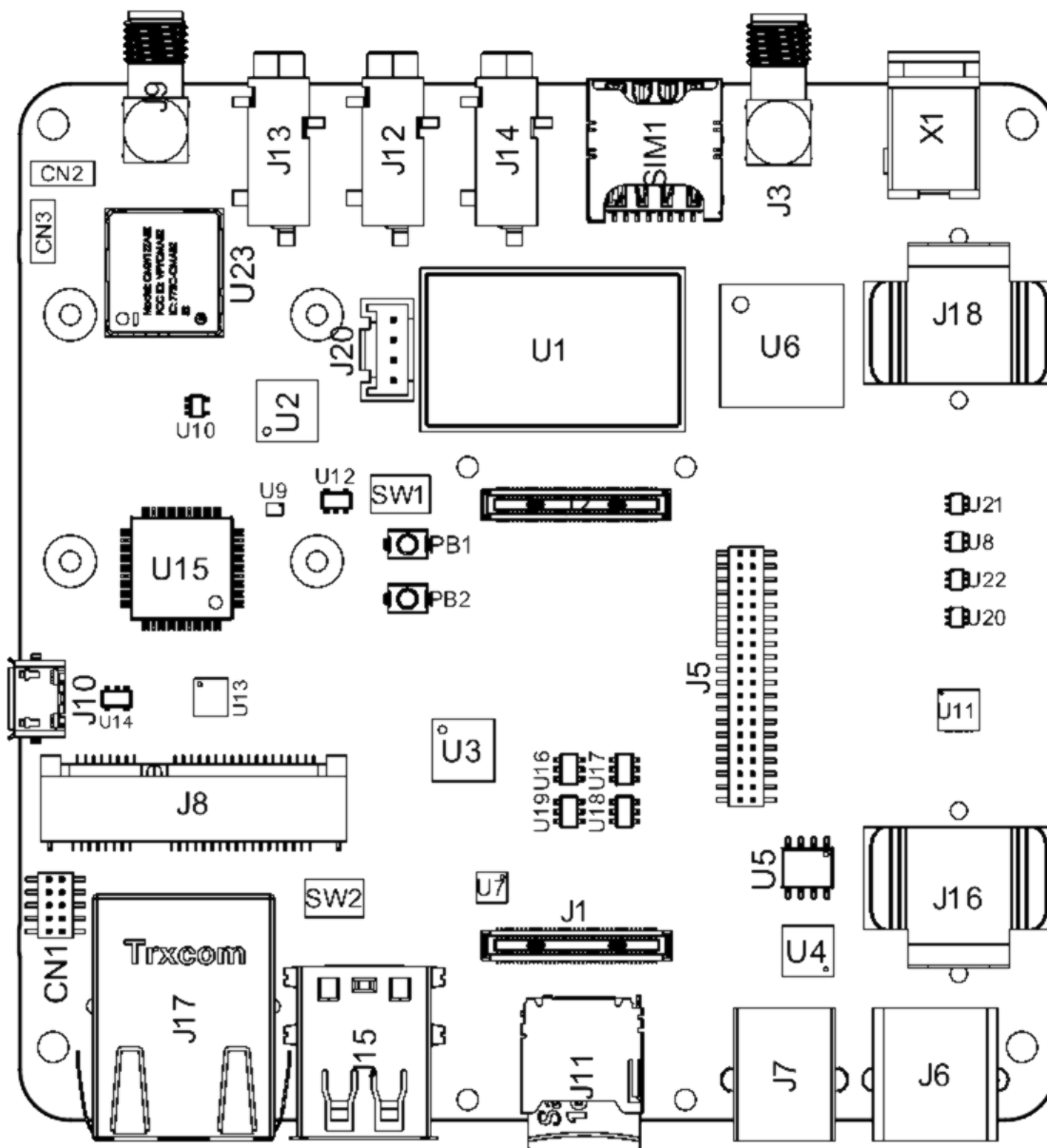
Board topology
