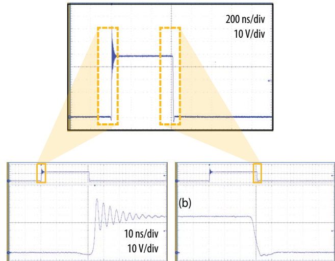
Figure 12: EPC9170 switch node waveform buck V_{IN} = 48 V, V_{OUT} = 14.3 V, I_{OUT} = 10 A
