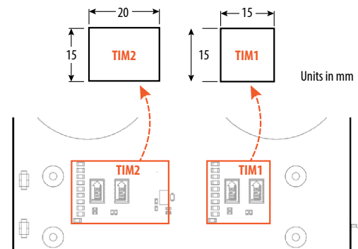
Figure 7. EPC9170 TIM specifications and location
