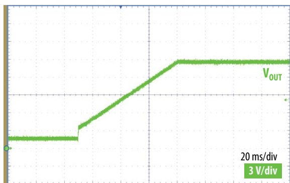
Figure 11: EPC9170 start up waveform buck V_{IN} = 48 V
