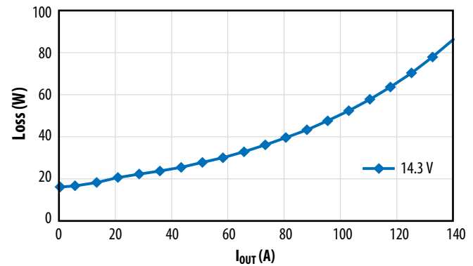
Figure 8: EPC9170 typical efficiency and power loss, buck V_{IN} = 48 V
