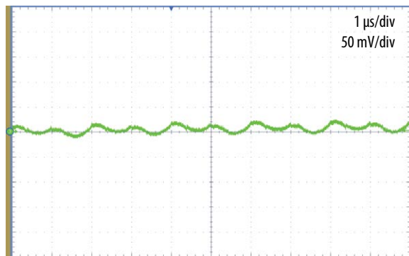
Figure 9: EPC9170 output voltage ripple buck V_{IN} = 48 V, V_{OUT} = 14.3 V, I_{OUT} = 21 A
