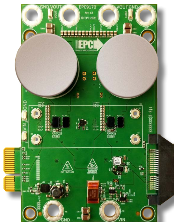
EPC9170 demonstration board
