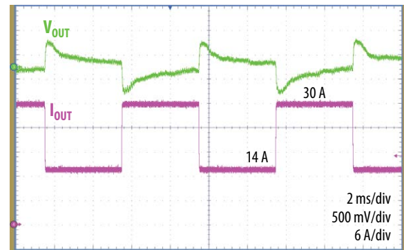
Figure 10: EPC9170 transient response buck V_{IN} = 48 V, V_{OUT} = 14.3 V
