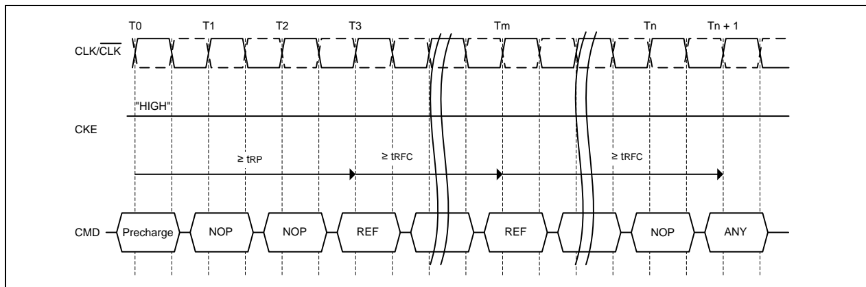
Figure 13 – Refresh command
