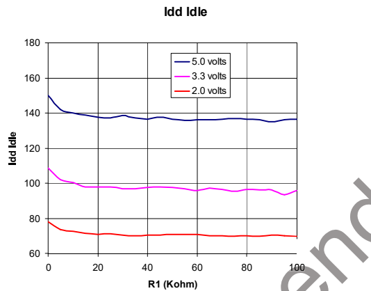
Figure 5. Idle Supply Current vs. R1 (R2 = 0 k \Omega , Vtxo = 1 V)
