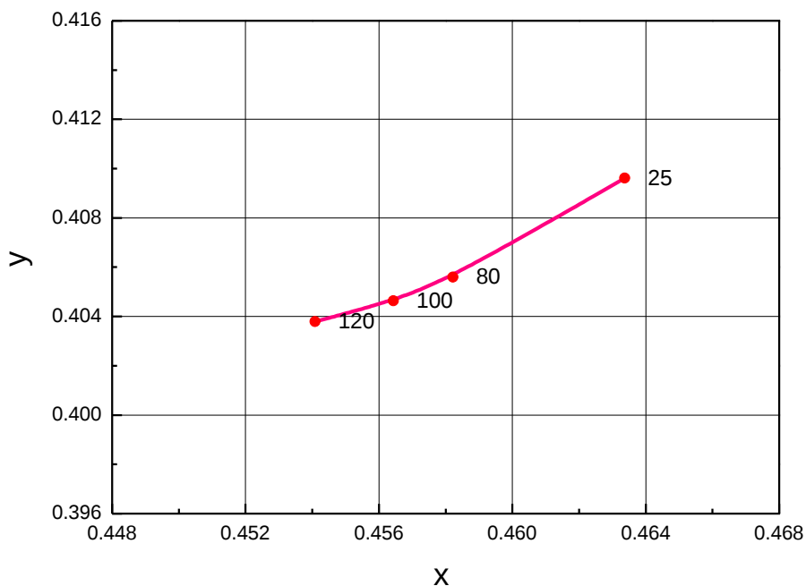
Fig 8. Chromaticity Coordinate vs. Junction Temperature, I_F=65\text{mA} (2600~4200K)
