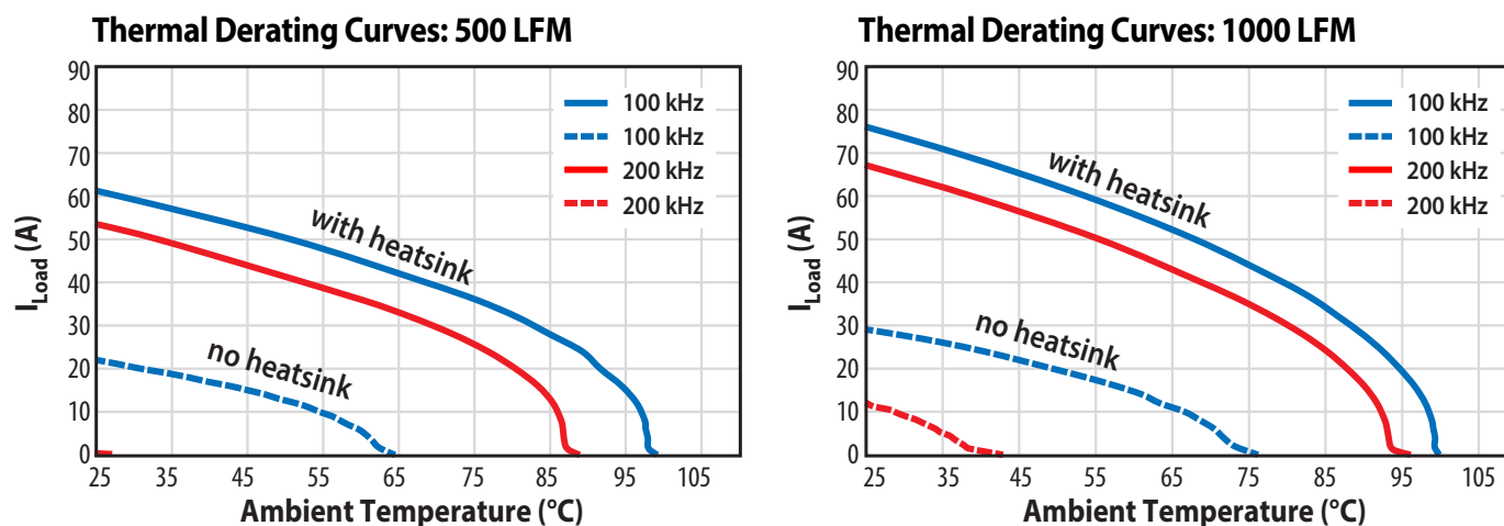
Figure 19: Typical thermal derating curve for two air flow rates, with and without a heatsink attached, measured with the board operating at various switching frequencies and using a 47 \mu H inductor
