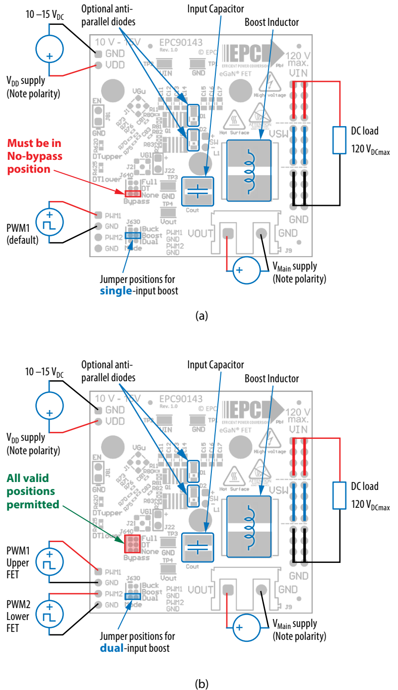
Figure 8: (a) Single-PWM input boost converter (b) Dual-PWM input boost converter configurations showing the supply, inductor, anti-parallel diodes, input capacitor, PWM, and load connections with corresponding jumper settings.
