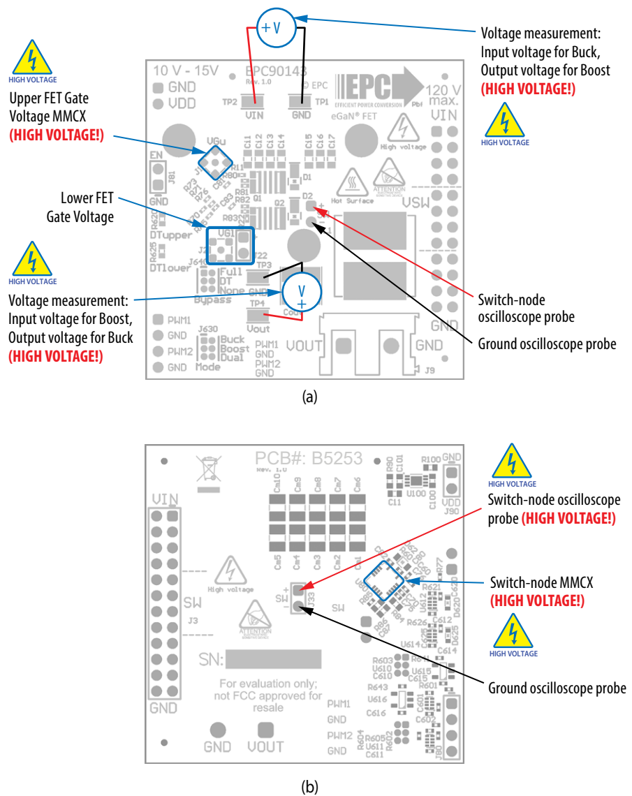
Figure 9: Measurement points (a) top side, (b) bottom side
