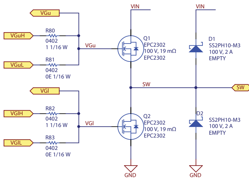
Power Stage
