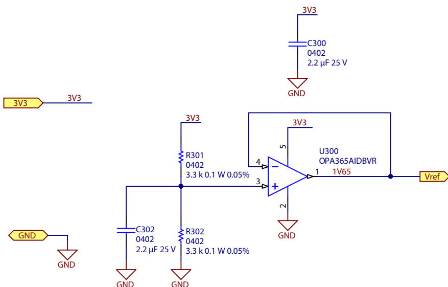
Figure 20: EPC9165 1.65 V reference schematic
