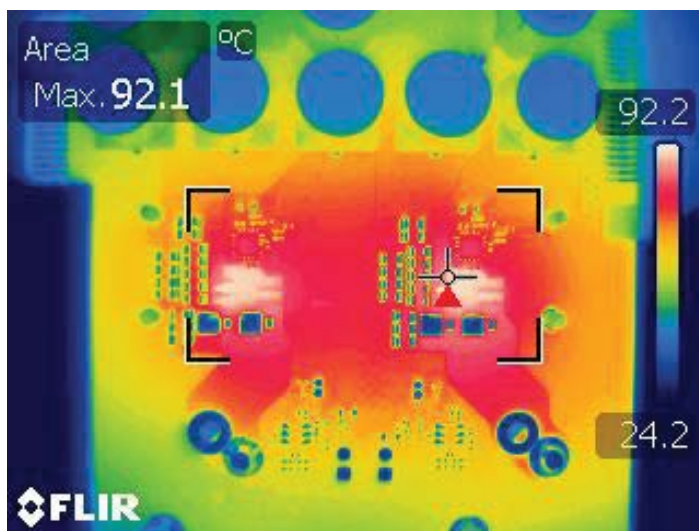
Figure 12. Thermal image showing FET region (back side of the board) temperature at full load with heatsink and 2000 LFM forced air cooling
