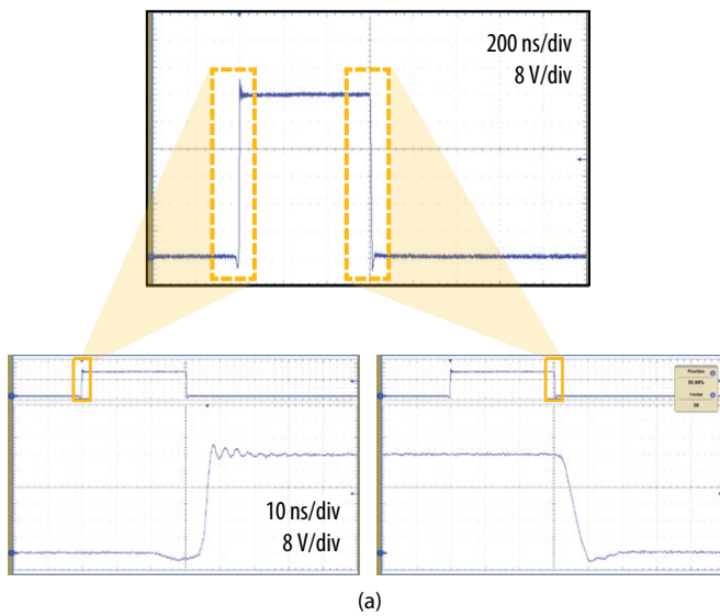
Figure 11: EPC9165 switch node waveform (a) buck V_{IN} = 48\text{ V} ; (b) boost V_{IN} = 14.3\text{ V}
