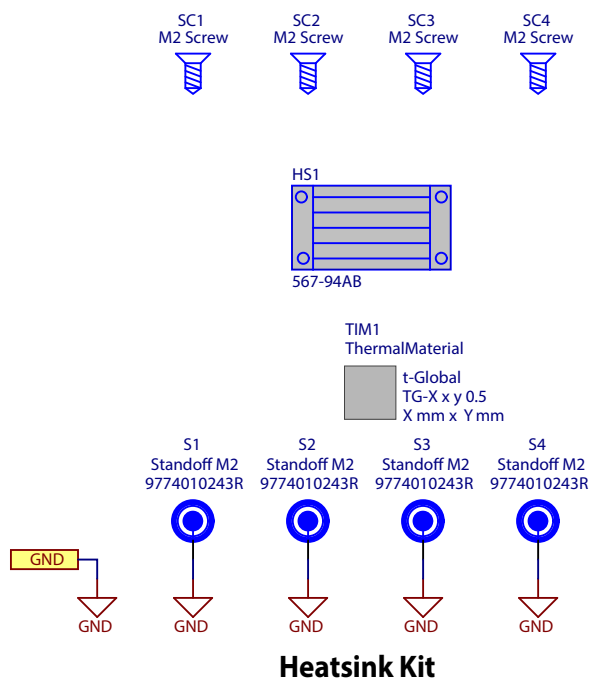
Figure 22: EPC9165 heatsink kit schematic
