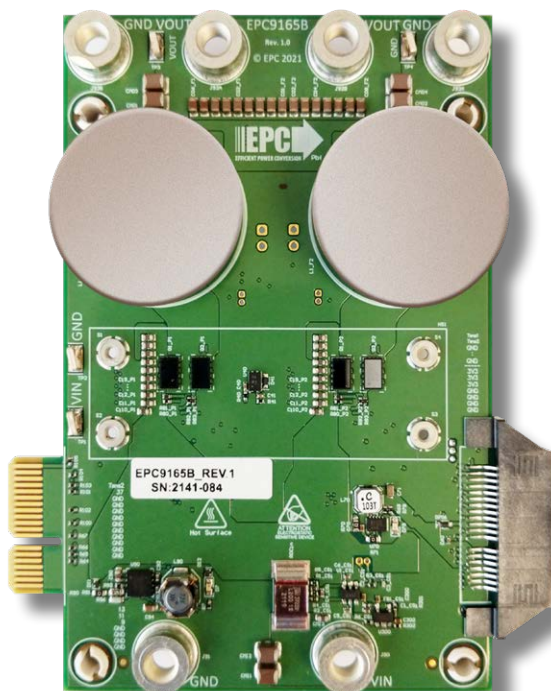
EPC9165 demonstration board
