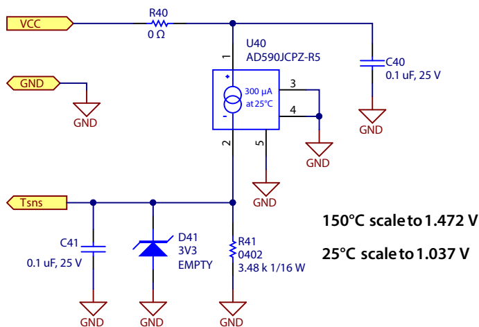
Figure 21: EPC9165 AD590 temperature sense schematic
